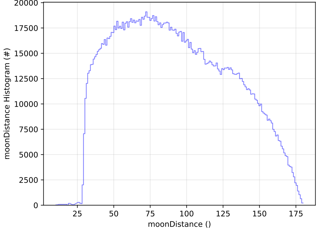
ddf_acor_sf10_lsf40_lsr10_v3.4_10yrs All sky all bands: moonDistance Histogram
