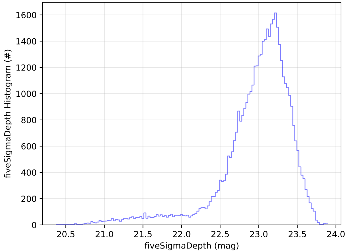
ddf_acor_sf10_lsf40_lsr10_v3.4_10yrs Yr 1 z band: fiveSigmaDepth Histogram
