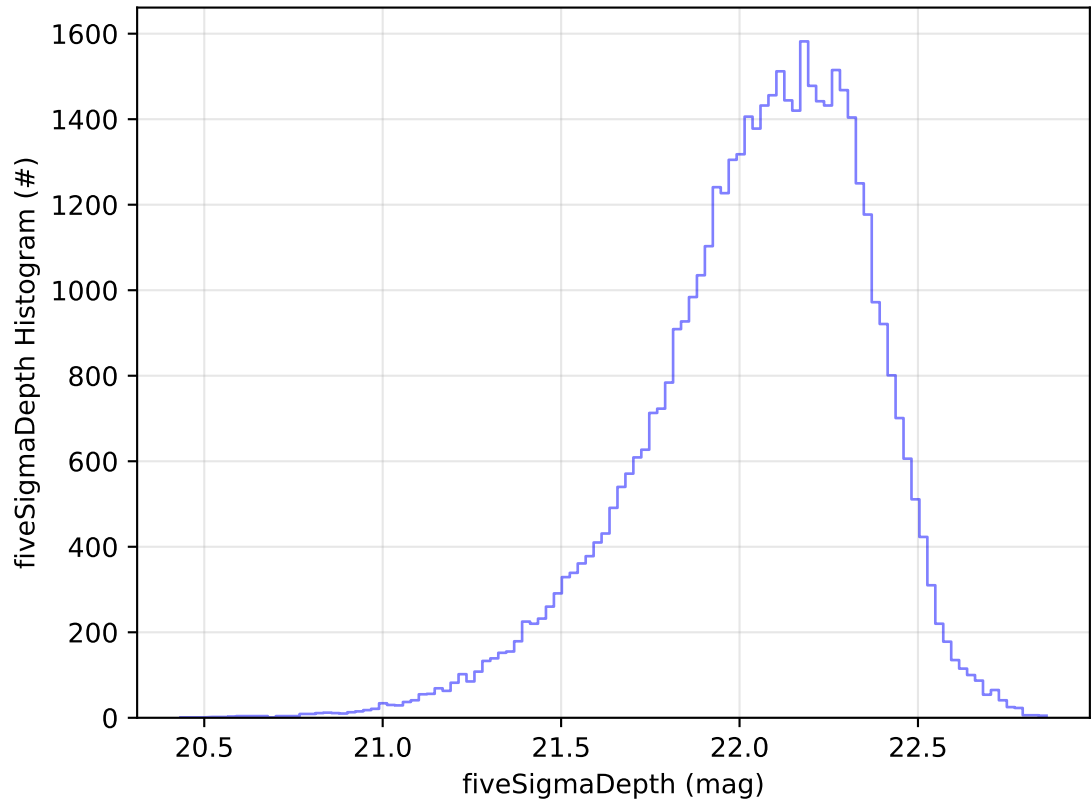
ddf_acor_sf10_lsf40_lsr10_v3.4_10yrs Yr 1 y band: fiveSigmaDepth Histogram
