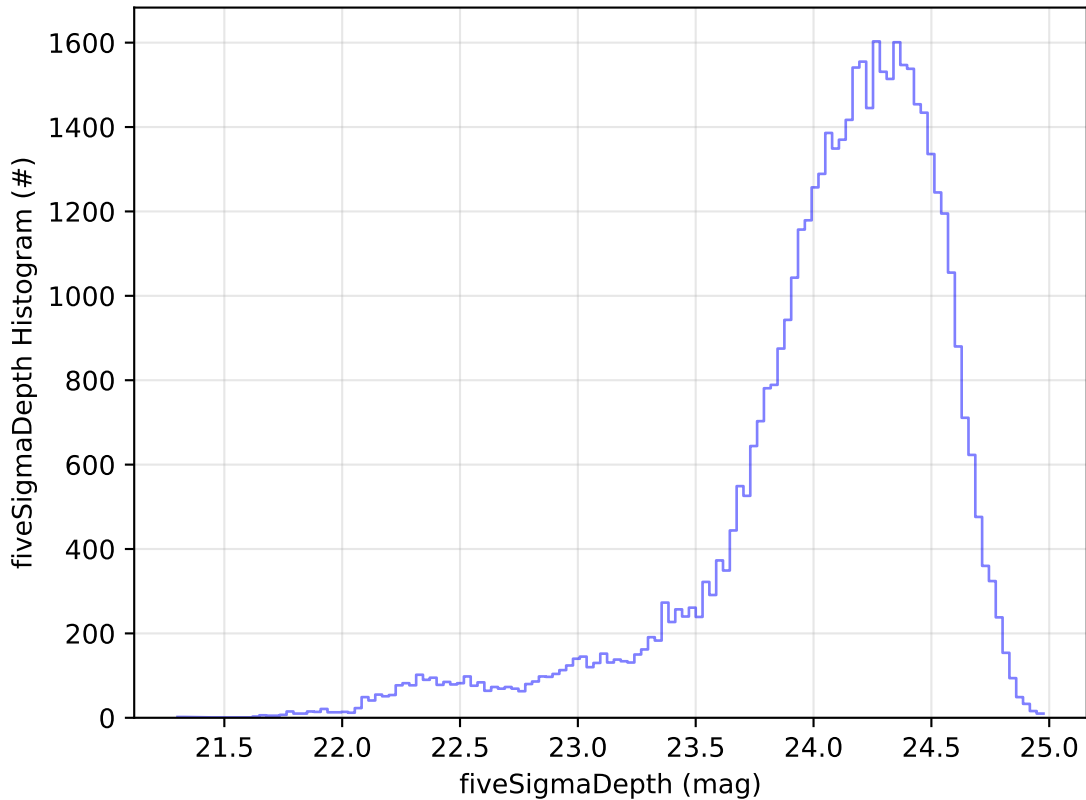
ddf_acor_sf10_lsf40_lsr10_v3.4_10yrs Yr 1 r band: fiveSigmaDepth Histogram
