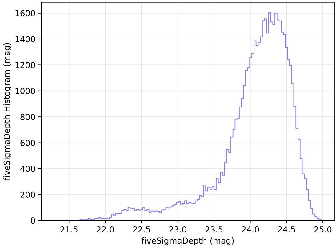
ddf_acor_sf10_ls40_lsr10_v3.4_10yrs Yr 1 r band: fiveSigmaDepth Histogram
