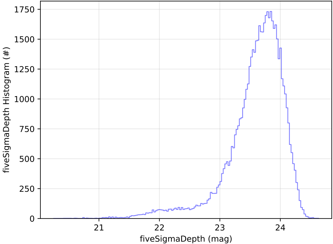
ddf_acor_sf10_lsf40_lsr10_v3.4_10yrs Yr 1 i band: fiveSigmaDepth Histogram
