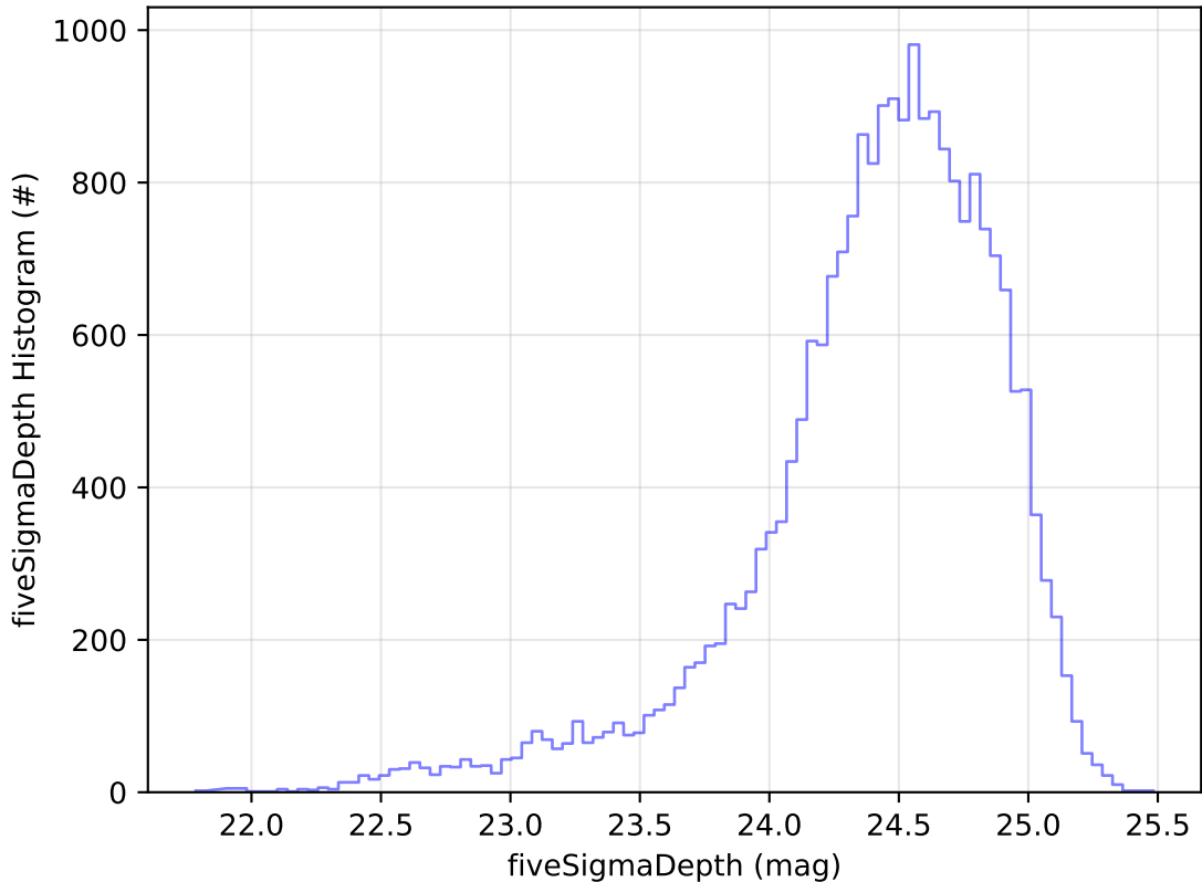
ddf_acor_sf10_lsf40_lsr10_v3.4_10yrs Yr 1 g band: fiveSigmaDepth Histogram
