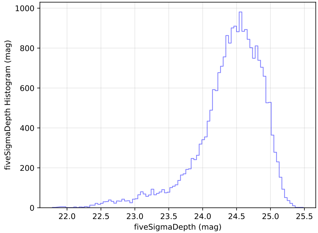
ddf_acor_sf10_lsf40_lsr10_v3.4_10yrs Yr 1 g band: fiveSigmaDepth Histogram
