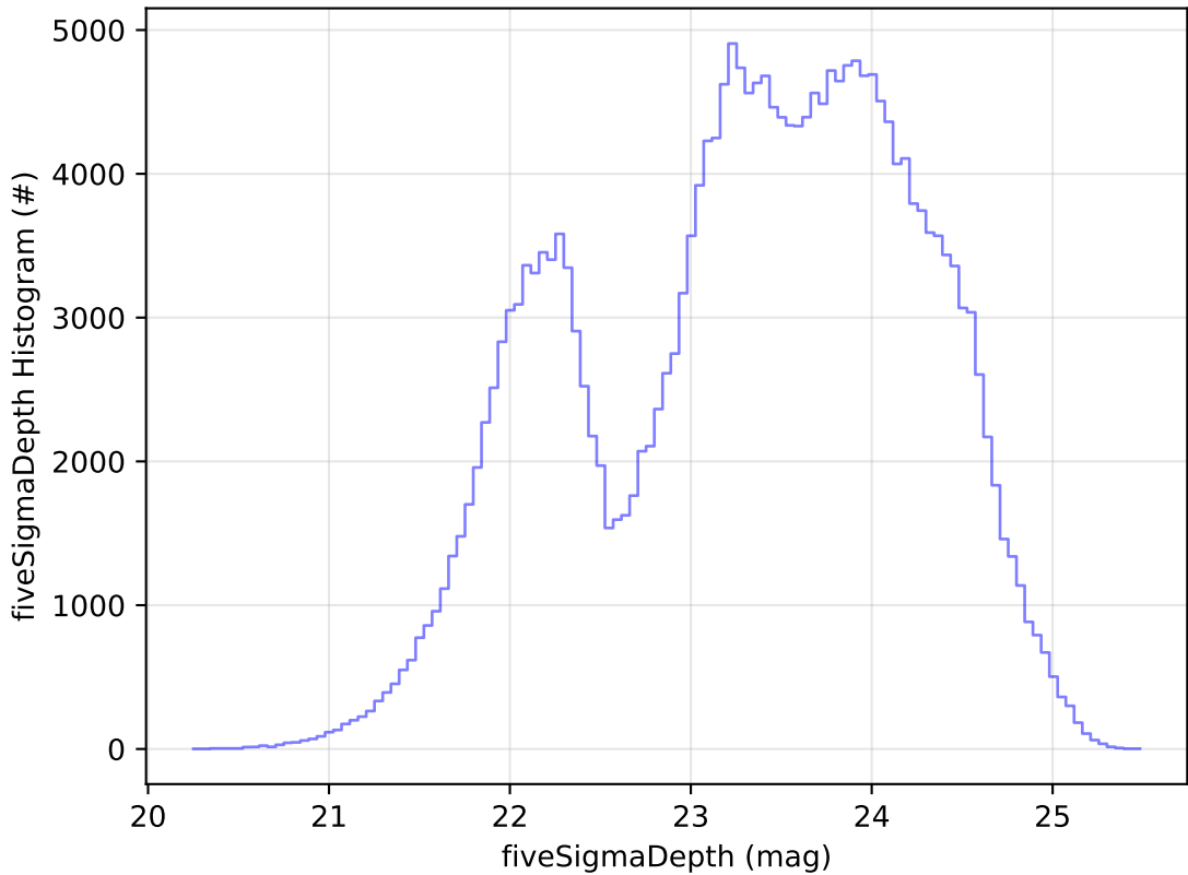
ddf_acor_sf10_lsf40_lsr10_v3.4_10yrs Yr 1 all bands: fiveSigmaDepth Histogram
