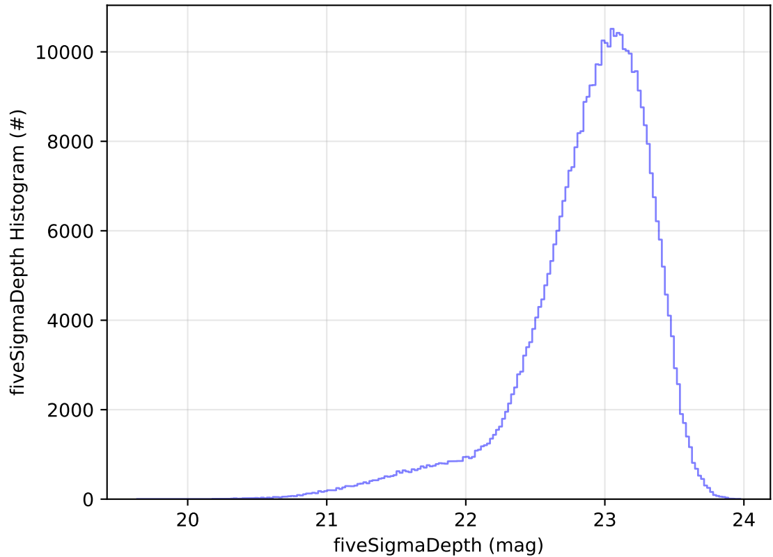
ddf_acor_sf10_lsf40_lsr10_v3.4_10yrs WFD z band: fiveSigmaDepth Histogram
