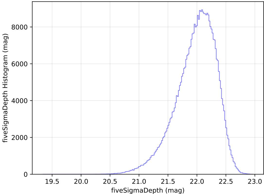
ddf_acor_sf10_lsf40_lsr10_v3.4_10yrs WFD y band: fiveSigmaDepth Histogram
