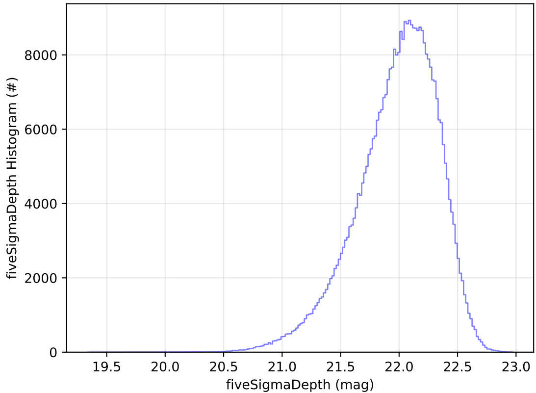
ddf_acor_sf10_ls40_lsr10_v3.4_10yrs WFD y band: fiveSigmaDepth Histogram
