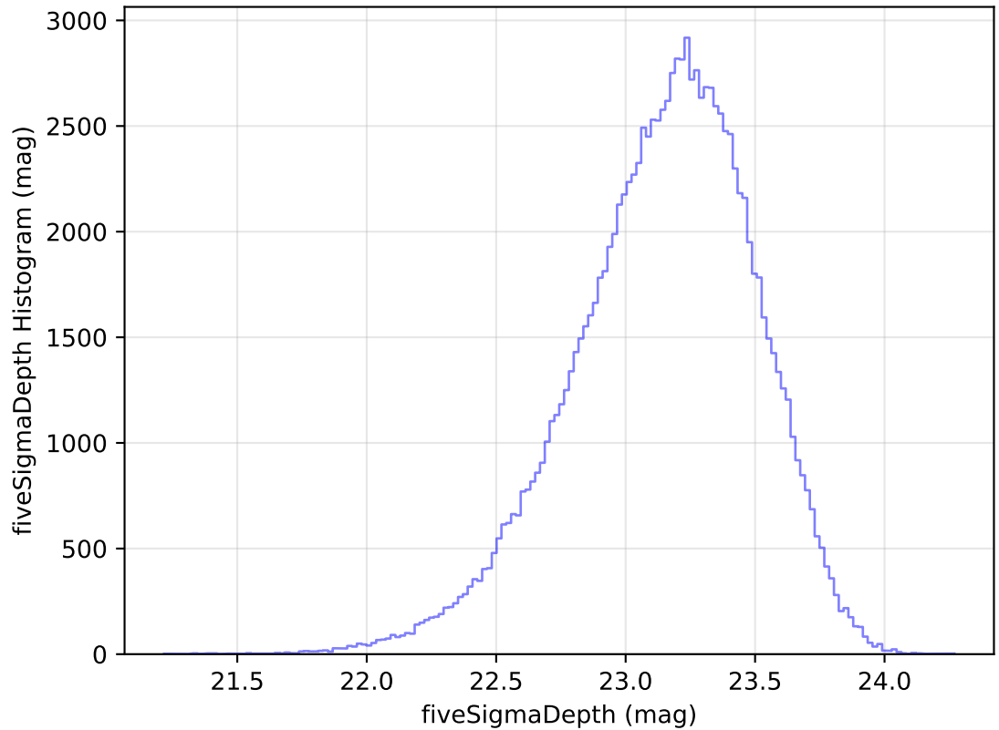
ddf_acor_sf10_lsf40_lsr10_v3.4_10yrs WFD u band: fiveSigmaDepth Histogram
