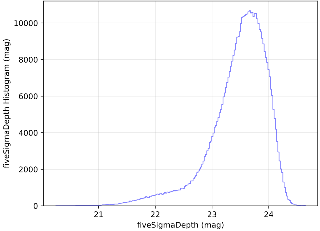
ddf_acor_sf10_lsf40_lsr10_v3.4_10yrs WFD i band: fiveSigmaDepth Histogram
