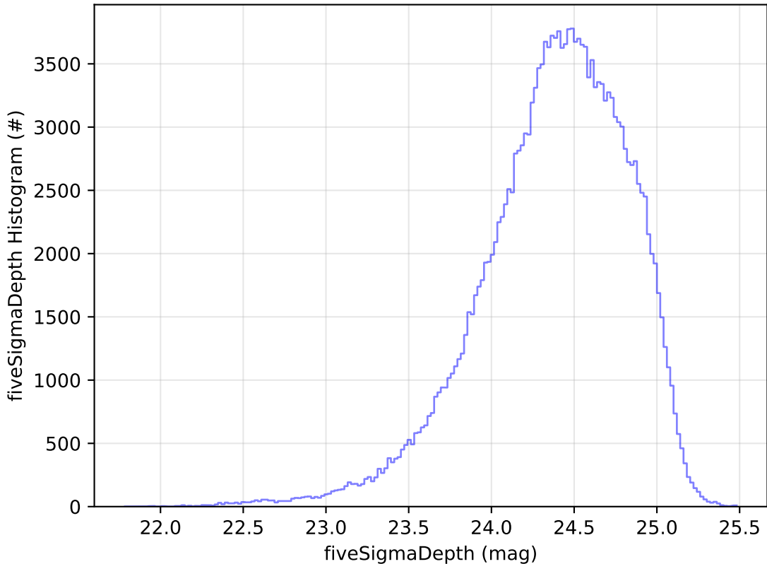
ddf_acor_sf10_ls40_lsr10_v3.4_10yrs WFD g band: fiveSigmaDepth Histogram
