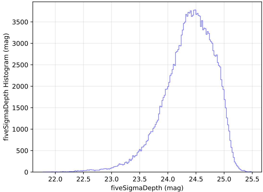
ddf_acor_sf10_lsf40_lsr10_v3.4_10yrs WFD g band: fiveSigmaDepth Histogram
