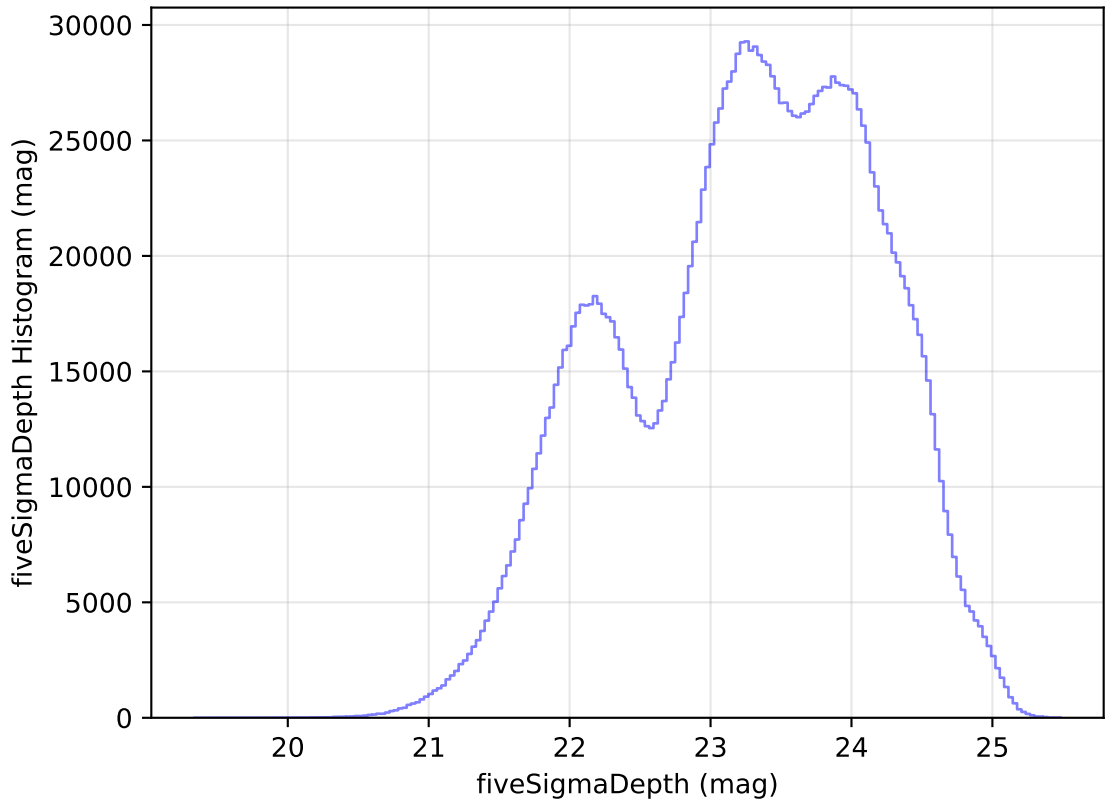
ddf_acor_sf10_lsf40_lsr10_v3.4_10yrs WFD all bands: fiveSigmaDepth Histogram
