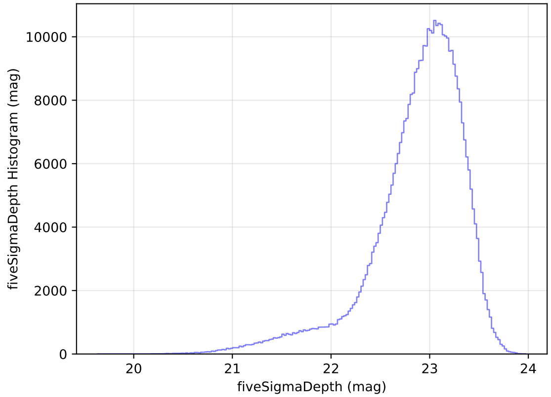
ddf_acor_sf10_lsf40_lsr10_v3.4_10yrs All sky z band: fiveSigmaDepth Histogram
