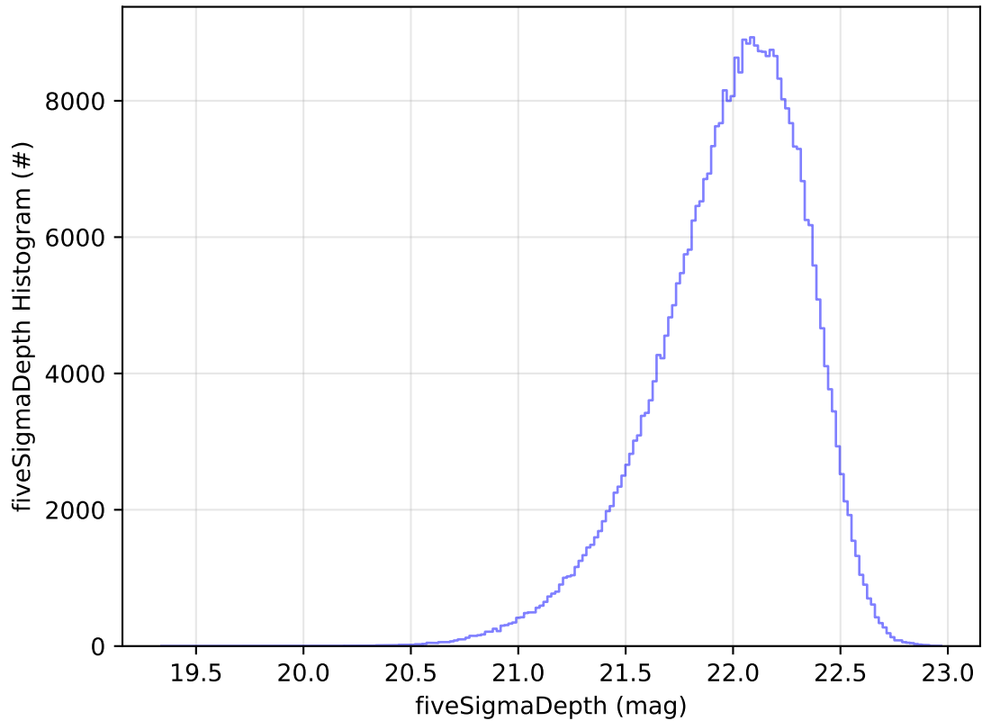
ddf_acor_sf10_lsf40_lsr10_v3.4_10yrs All sky y band: fiveSigmaDepth Histogram
