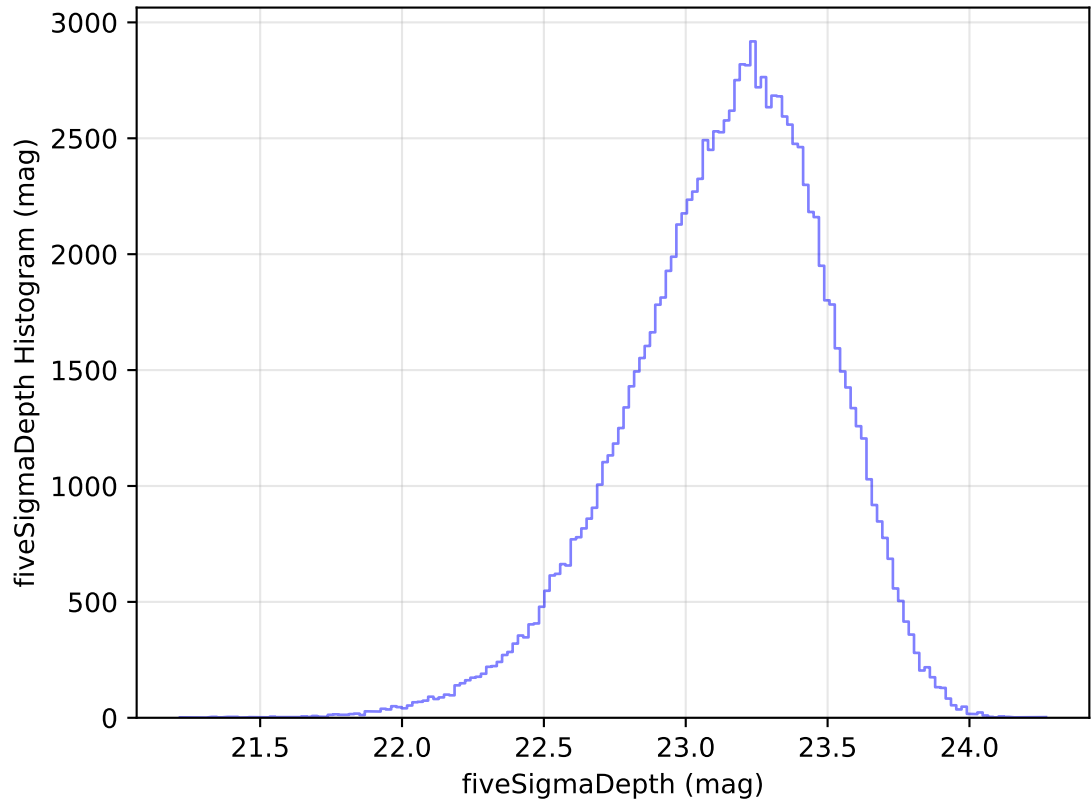
ddf_acor_sf10_lsf40_lsr10_v3.4_10yrs All sky u band: fiveSigmaDepth Histogram
