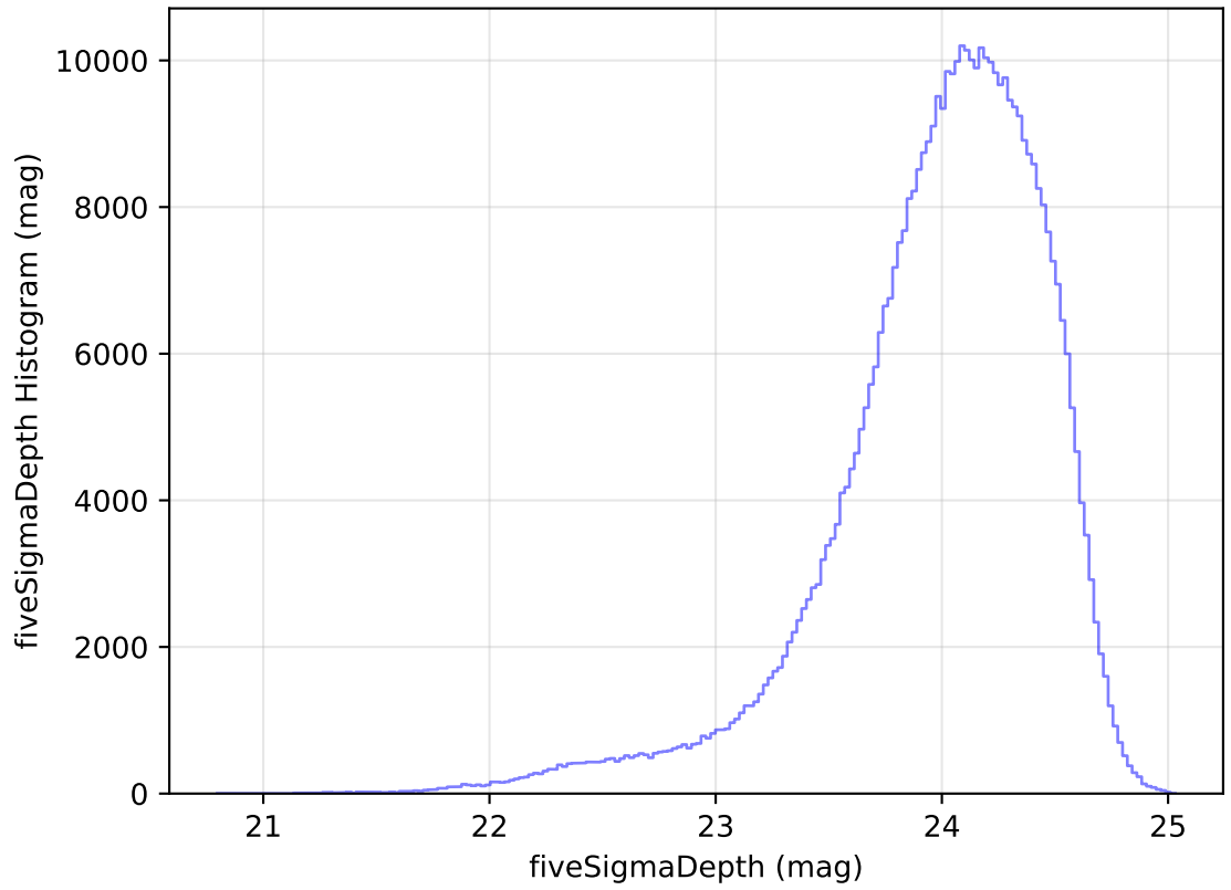
ddf_acor_sf10_lsf40_lsr10_v3.4_10yrs All sky r band: fiveSigmaDepth Histogram
