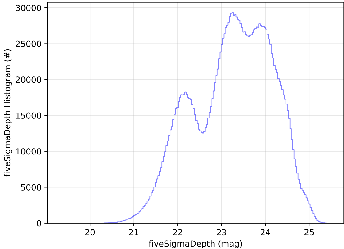
ddf_acor_sf10_lsf40_lsr10_v3.4_10yrs All sky all bands: fiveSigmaDepth Histogram
