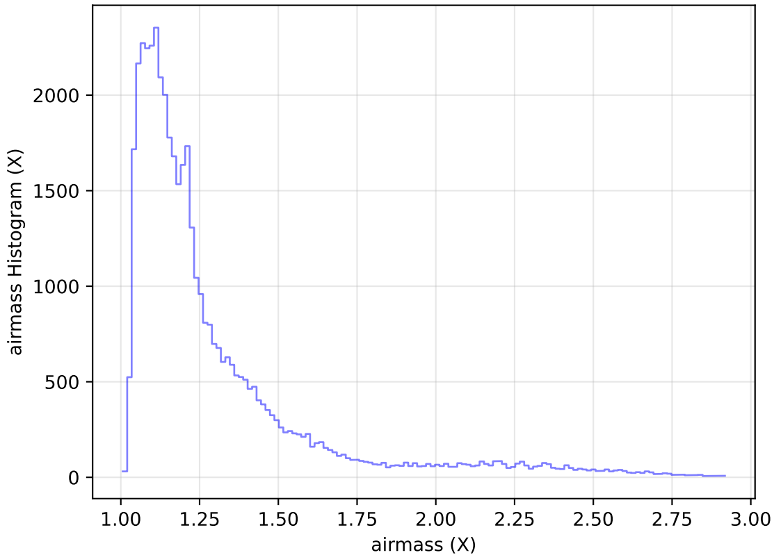
ddf_acor_sf10_lsf40_lsr10_v3.4_10yrs Yr 1 z band: airmass Histogram
