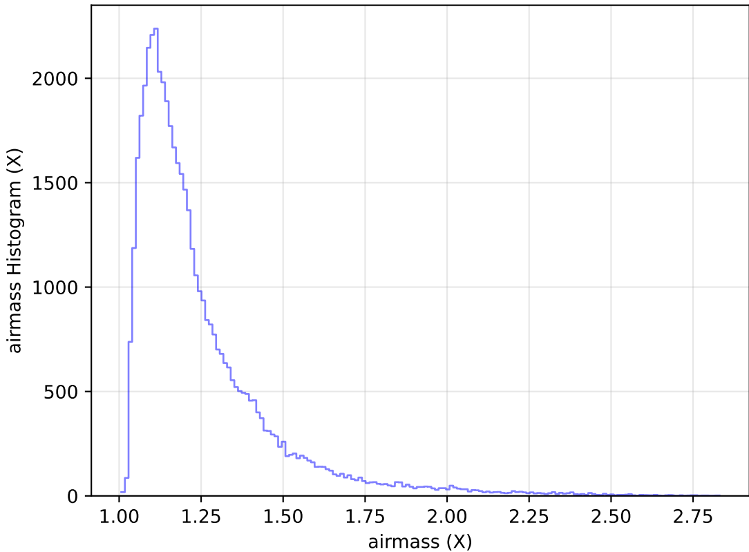
ddf_acor_sf10_lsf40_lsr10_v3.4_10yrs Yr 1 y band: airmass Histogram
