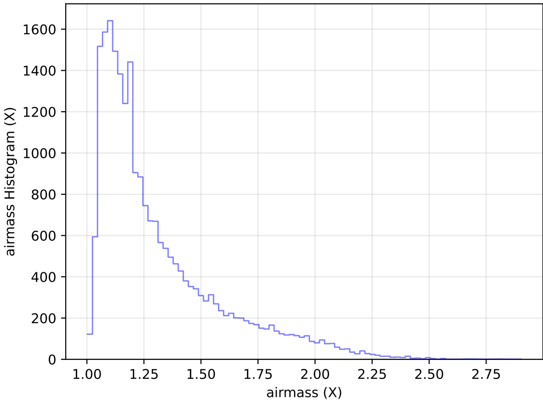
ddf_acor_sf10_lsf40_lsr10_v3.4_10yrs Yr 1 g band: airmass Histogram
