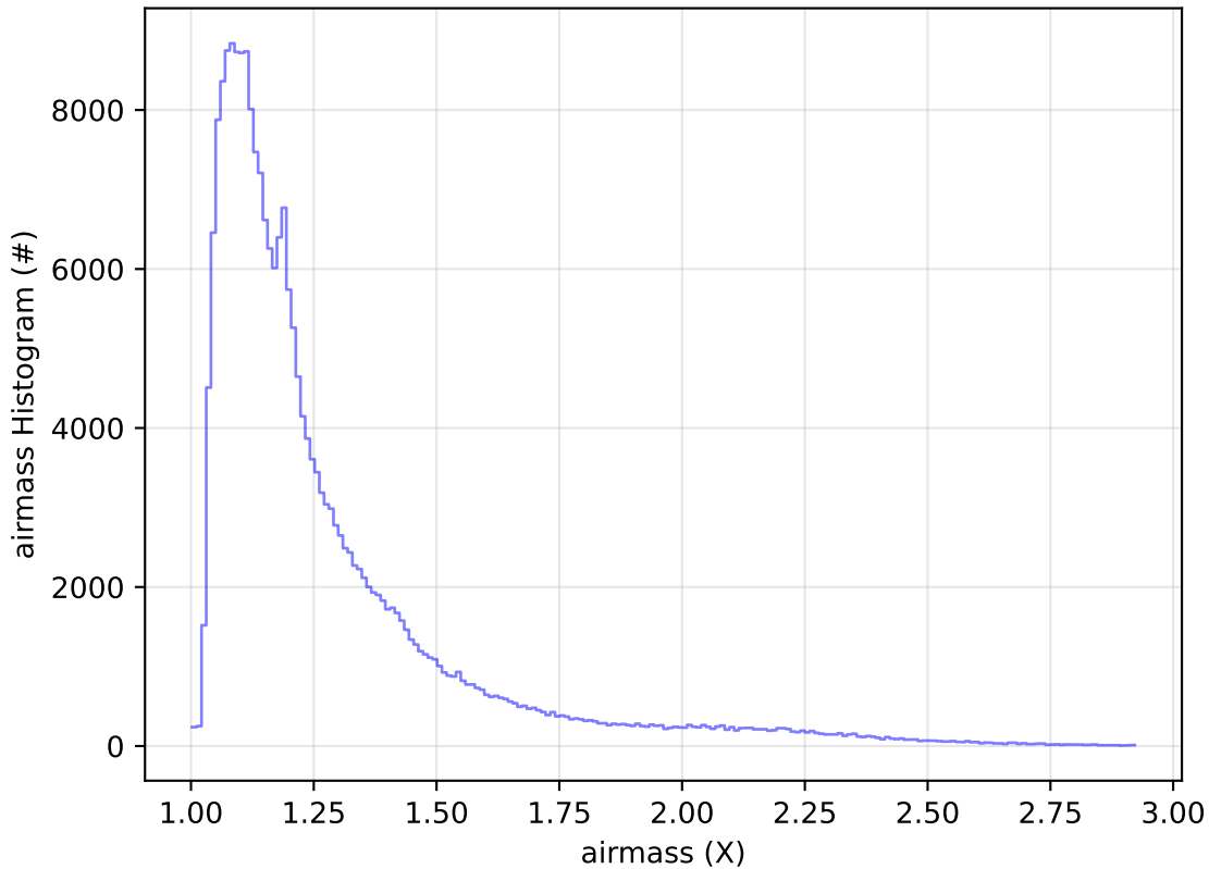
ddf_acor_sf10_lsf40_lsr10_v3.4_10yrs Yr 1 all bands: airmass Histogram
