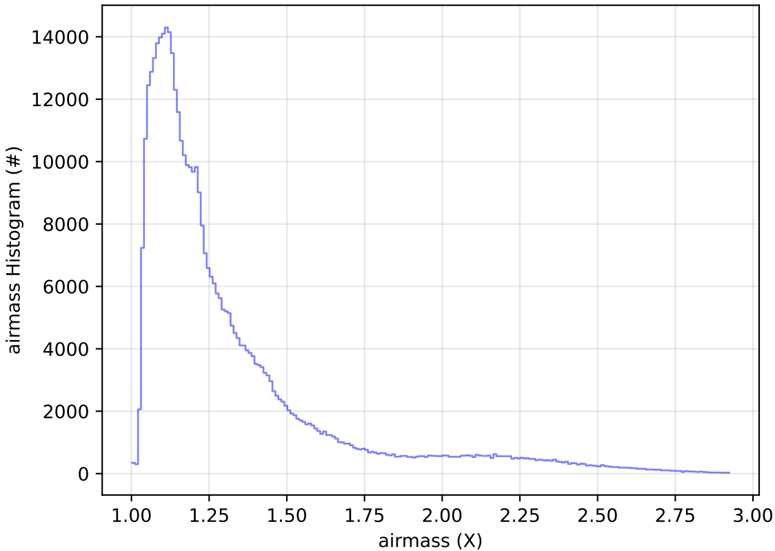
ddf_acor_sf10_lsf40_lsr10_v3.4_10yrs WFD z band: airmass Histogram
