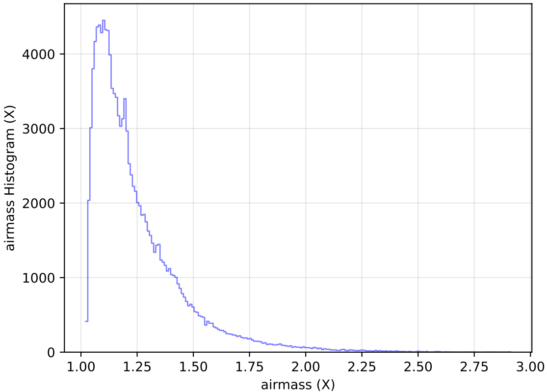
ddf_acor_sf10_lsf40_lsr10_v3.4_10yrs WFD u band: airmass Histogram
