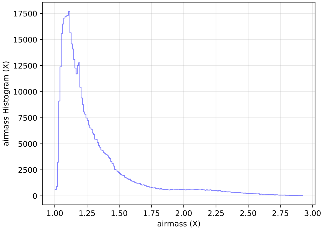
ddf_acor_sf10_lsf40_lsr10_v3.4_10yrs WFD i band: airmass Histogram
