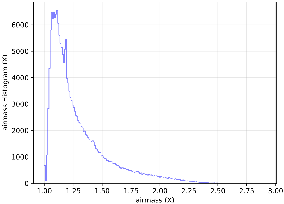
ddf_acor_sf10_lsf40_lsr10_v3.4_10yrs WFD g band: airmass Histogram
