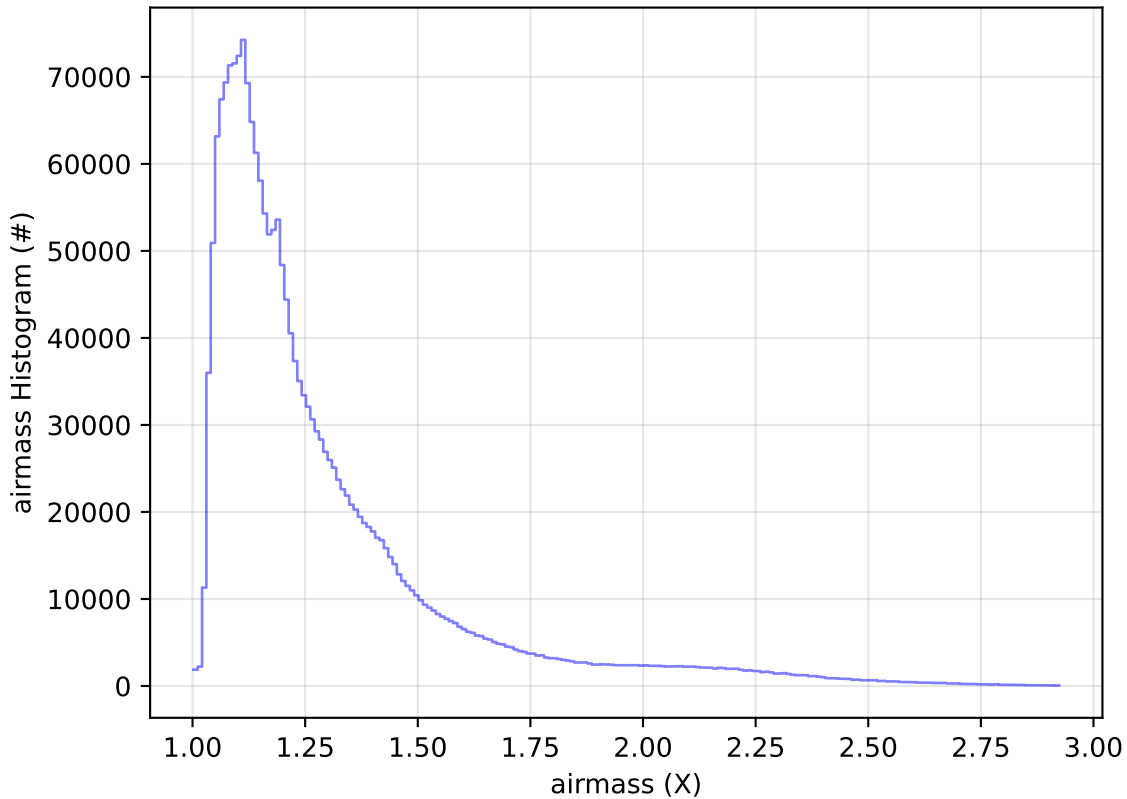
ddf_acor_sf10_lsf40_lsr10_v3.4_10yrs WFD all bands: airmass Histogram
