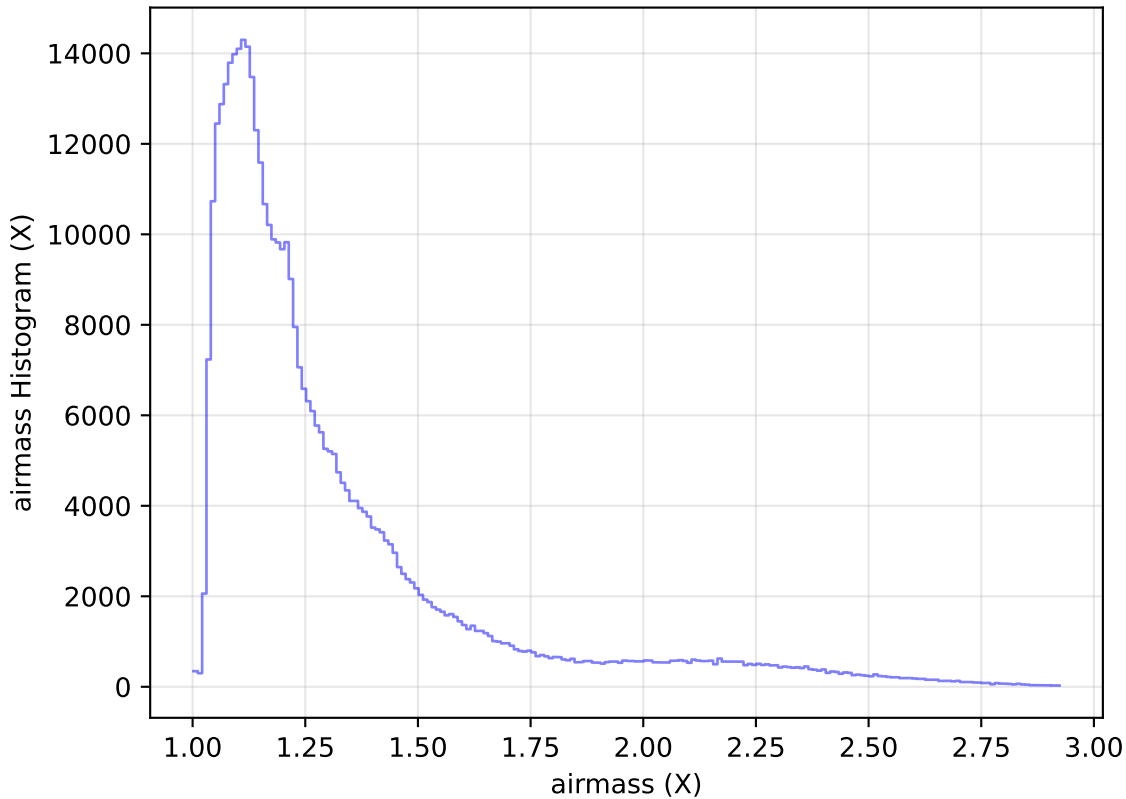
ddf_acor_sf10_lsf40_lsr10_v3.4_10yrs All sky z band: airmass Histogram
