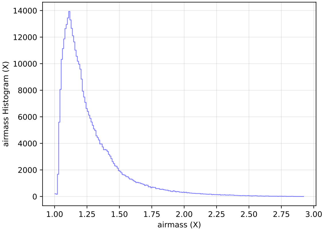
ddf_acor_sf10_lsf40_lsr10_v3.4_10yrs All sky y band: airmass Histogram
