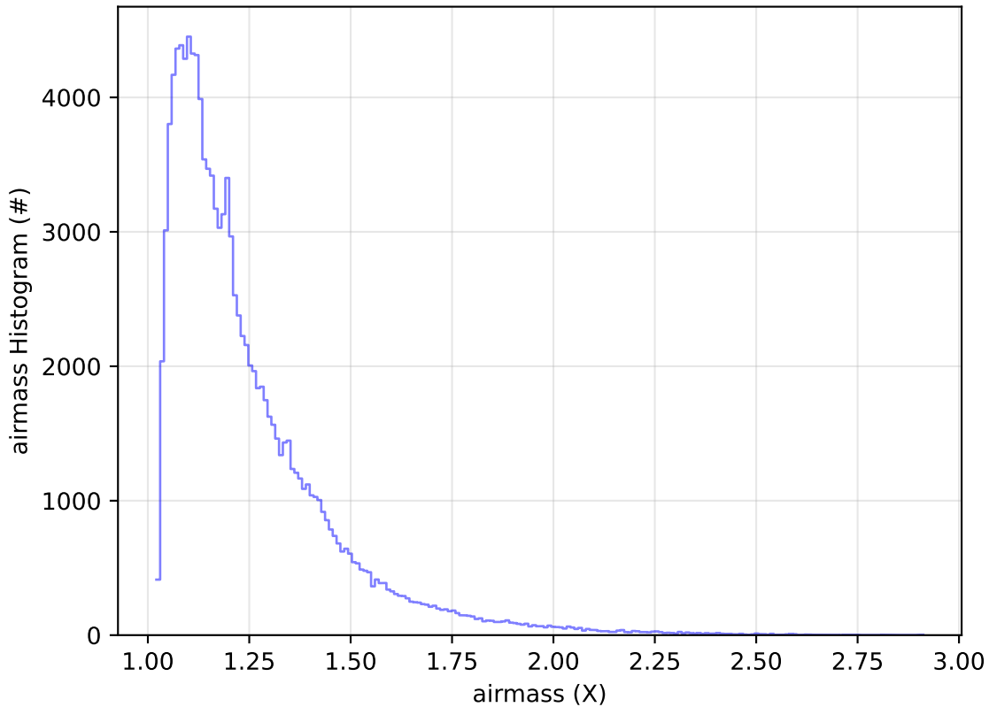
ddf_acor_sf10_lsf40_lsr10_v3.4_10yrs All sky u band: airmass Histogram
