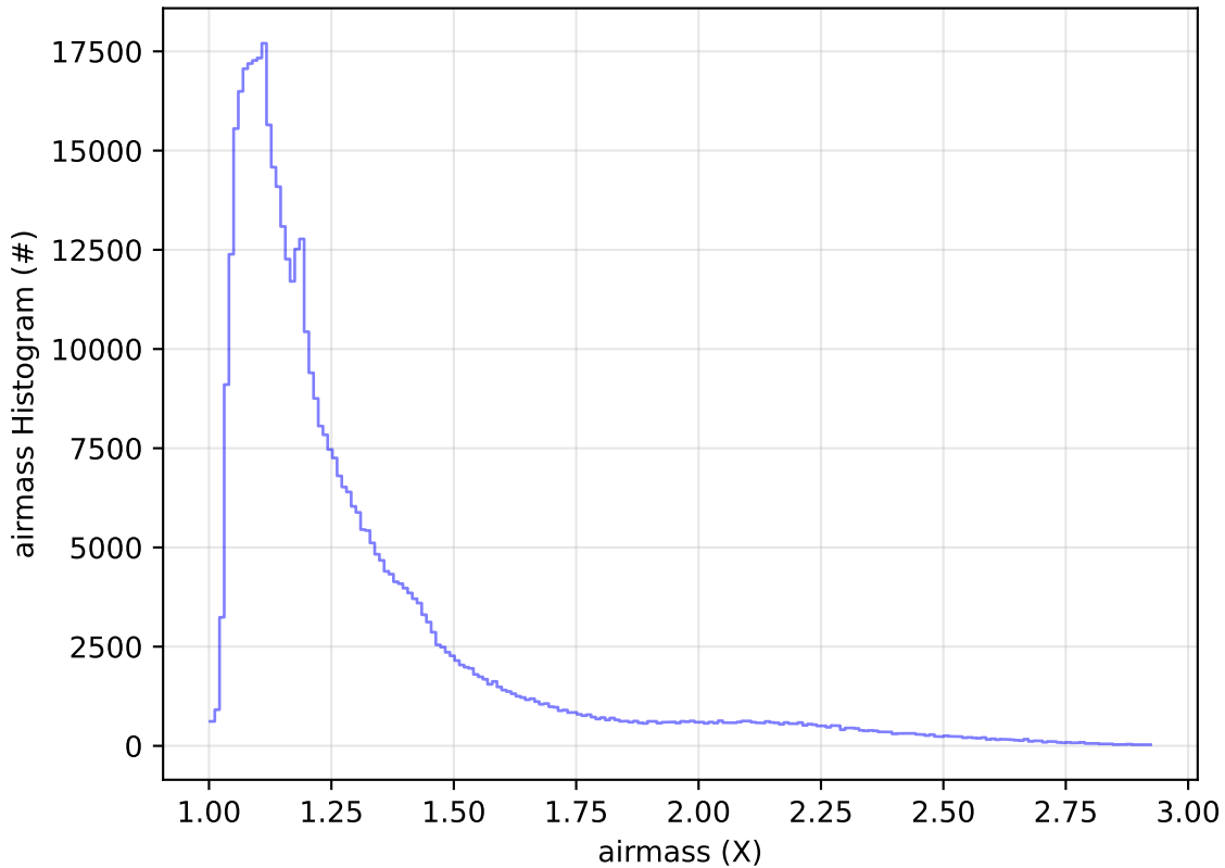
ddf_acor_sf10_lsf40_lsr10_v3.4_10yrs All sky i band: airmass Histogram
