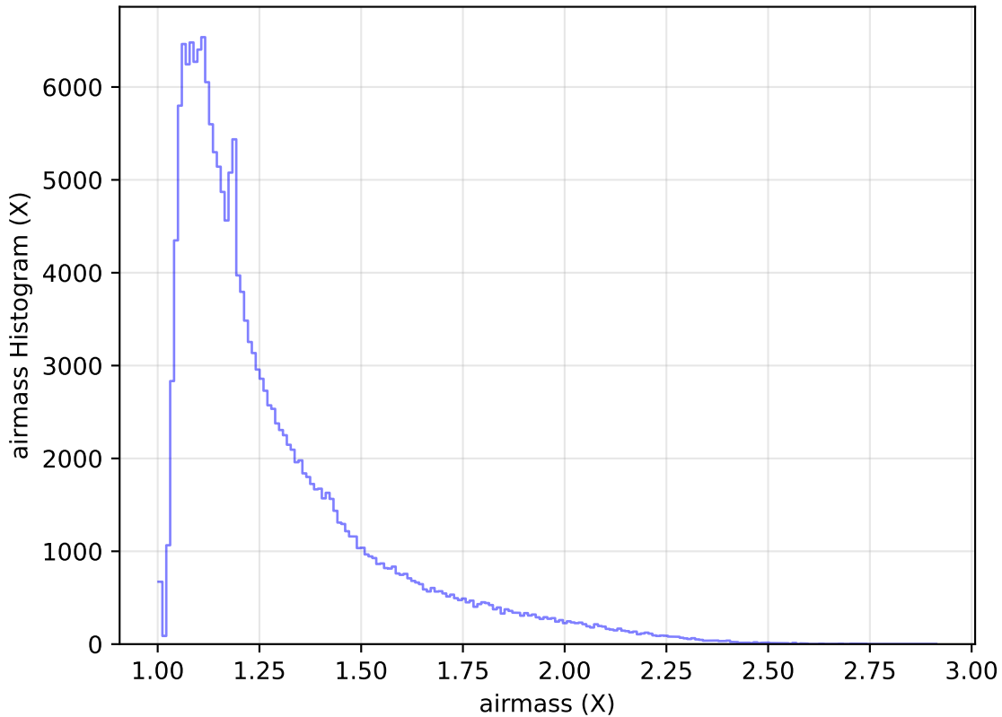
ddf_acor_sf10_lsf40_lsr10_v3.4_10yrs All sky g band: airmass Histogram
