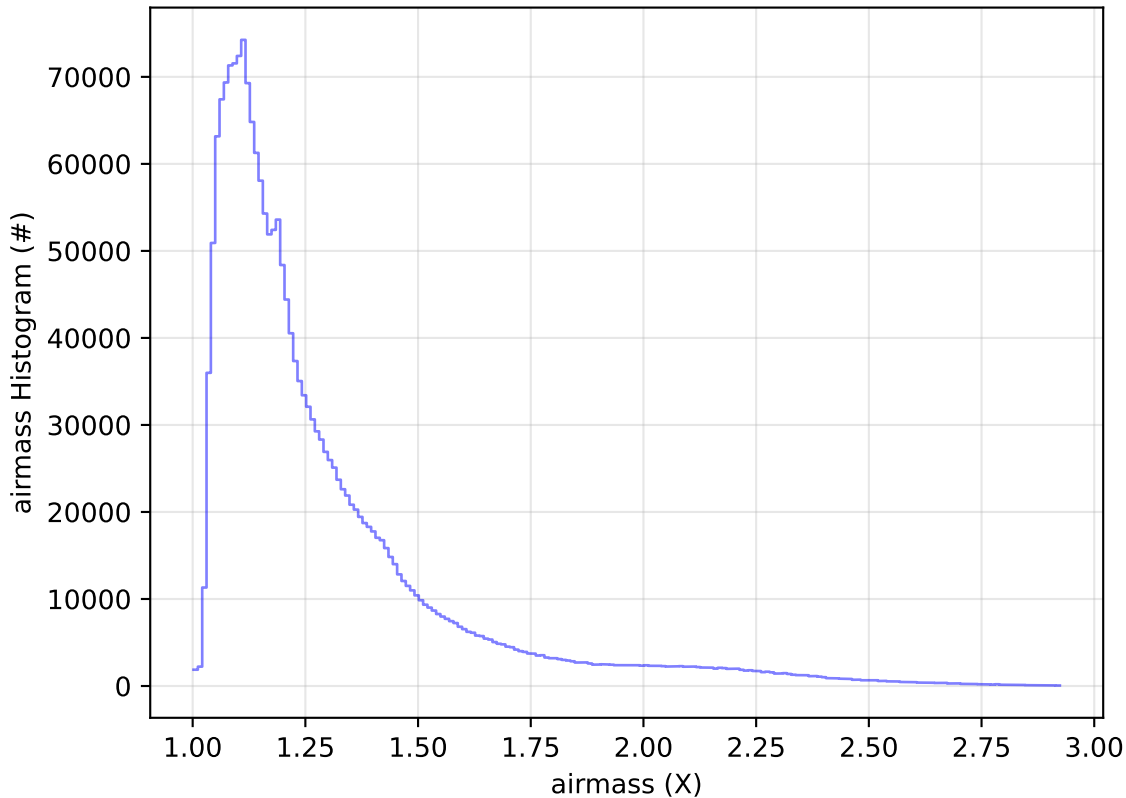
ddf_acor_sf10_lsf40_lsr10_v3.4_10yrs All sky all bands: airmass Histogram
