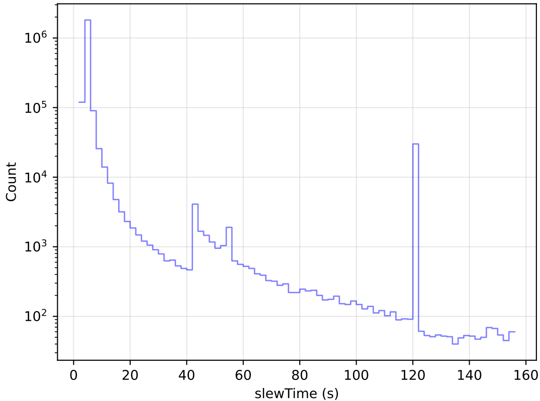
ddf_acor_sf10_lsf40_lsr10_v3.4_10yrs All visits: Slew Time Histogram
