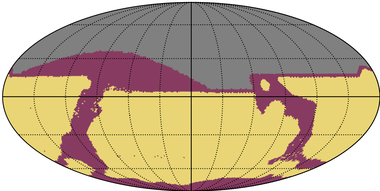
ddf_acor_sf10_lsf40_lsr10_v3.4_10yrs All sky: RapidRevisits
