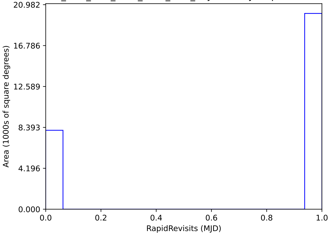
ddf_acor_sf10_lsf40_lsr10_v3.4_10yrs All sky: RapidRevisits
