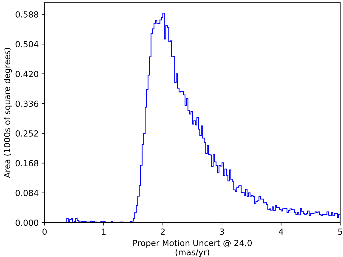
ddf_acor_sf10_lsf40_lsr10_v3.4_10yrs All sky: Proper Motion Uncert @ 24.0
