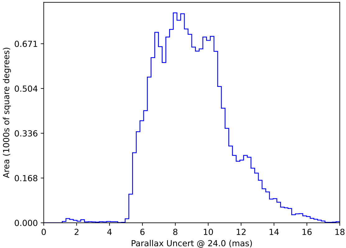
ddf_acor_sf10_lsf40_lsr10_v3.4_10yrs WFD: Parallax Uncert @ 24.0
