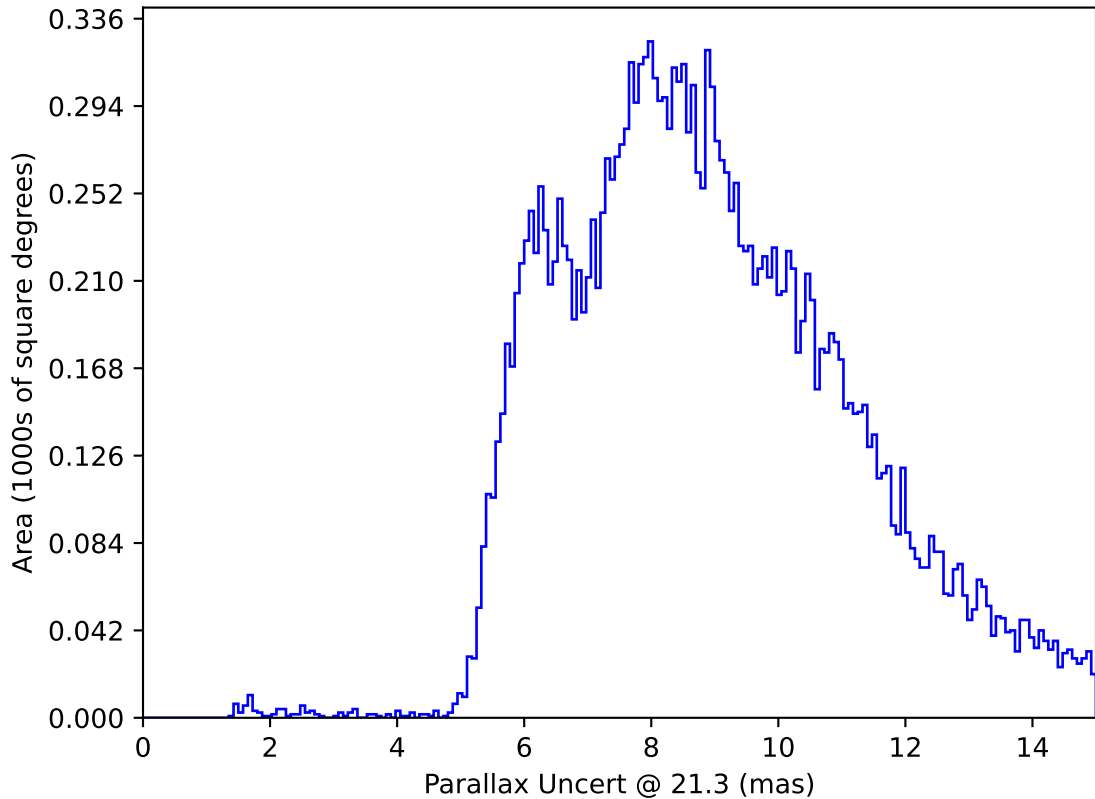
ddf_acor_sf10_lsf40_lsr10_v3.4_10yrs All sky y band only: Parallax Uncert @ 21.3
