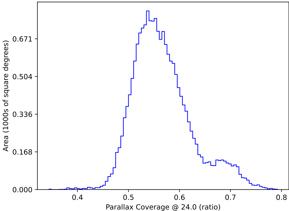
ddf_acor_sf10_lsf40_lsr10_v3.4_10yrs WFD: Parallax Coverage @ 24.0
