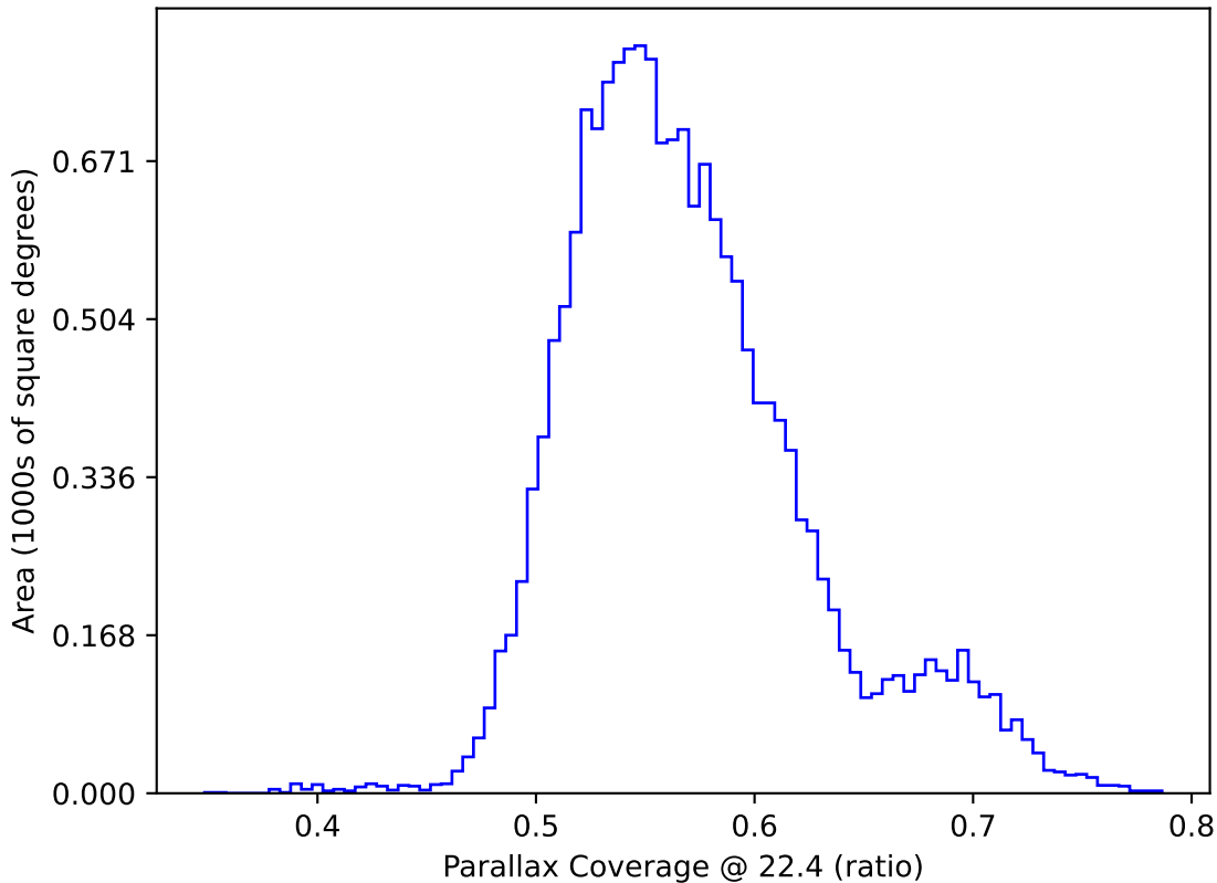
ddf_acor_sf10_lsf40_lsr10_v3.4_10yrs WFD: Parallax Coverage @ 22.4
