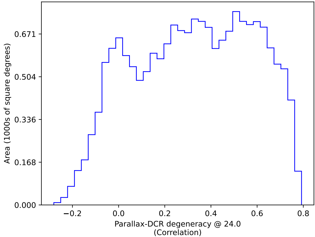
ddf_acor_sf10_lsf40_lsr10_v3.4_10yrs WFD: Parallax-DCR degeneracy @ 24.0
