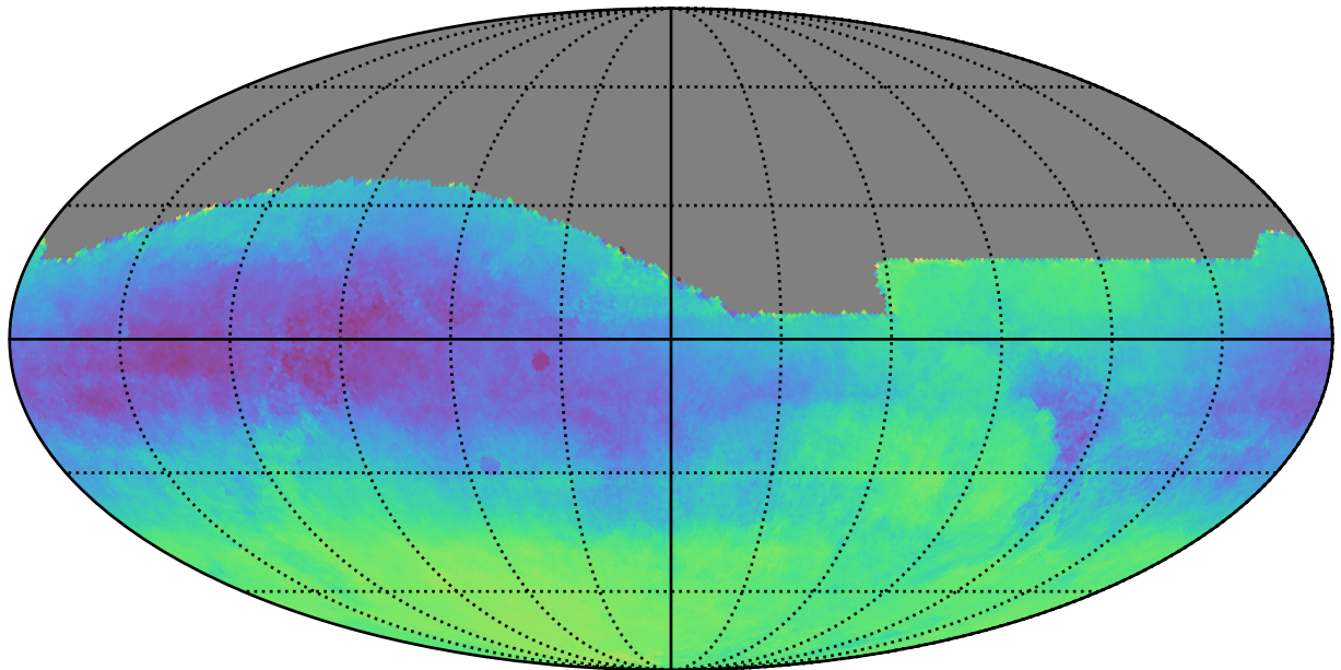
ddf_acor_sf10_lsf40_lsr10_v3.4_10yrs All sky: Parallax-DCR degeneracy @ 24.0
