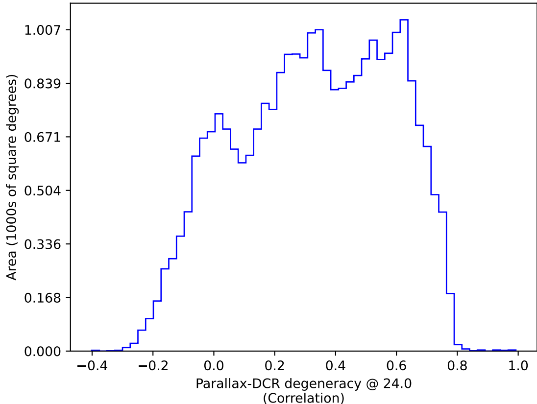
ddf_acor_sf10_lsf40_lsr10_v3.4_10yrs All sky: Parallax-DCR degeneracy @ 24.0
