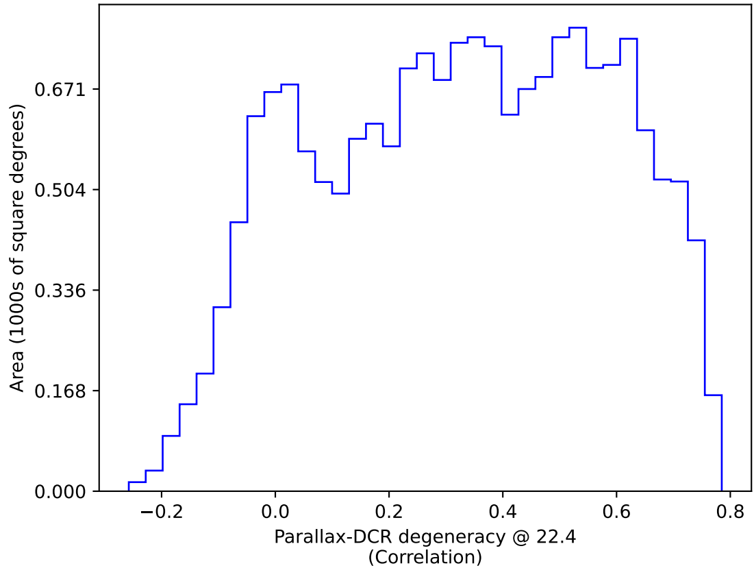
ddf_acor_sf10_lsf40_lsr10_v3.4_10yrs WFD: Parallax-DCR degeneracy @ 22.4
