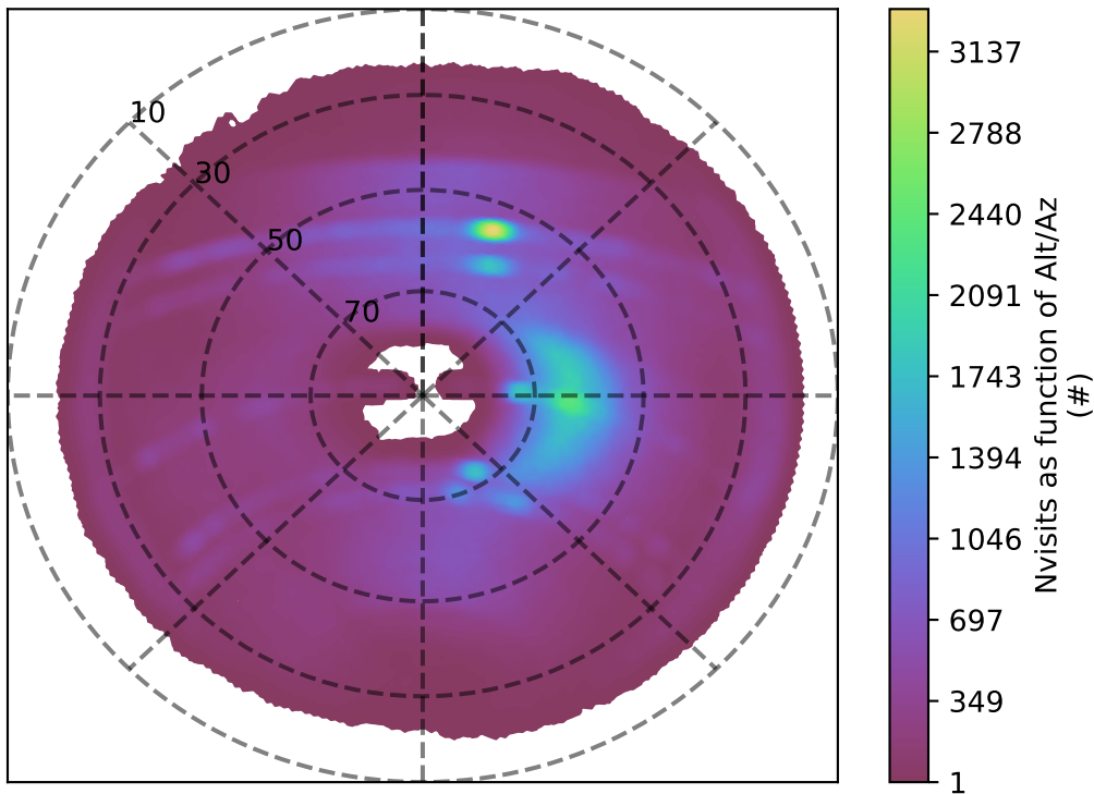
ddf_acor_sf10_lsf40_lsr10_v3.4_10yrs z band: Nvisits as function of Alt/Az
