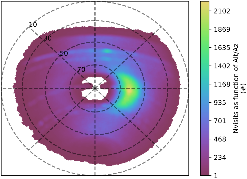
ddf_acor_sf10_lsf40_lsr10_v3.4_10yrs y band: Nvisits as function of Alt/Az
