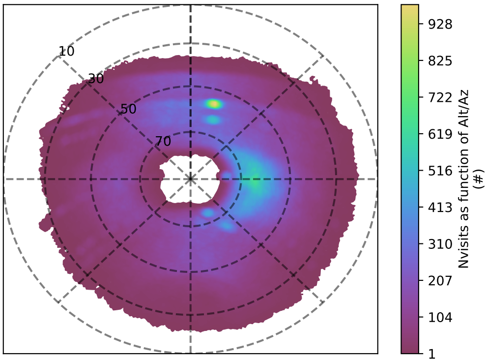
ddf_acor_sf10_lsf40_lsr10_v3.4_10yrs u band: Nvisits as function of Alt/Az
