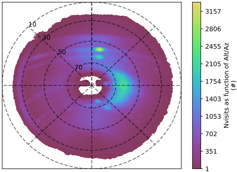
ddf_acor_sf10_lsf40_lsr10_v3.4_10yrs r band: Nvisits as function of Alt/Az
