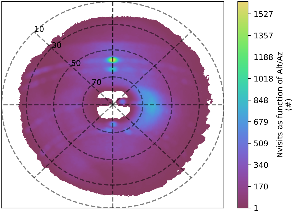
ddf_acor_sf10_lsf40_lsr10_v3.4_10yrs g band: Nvisits as function of Alt/Az
